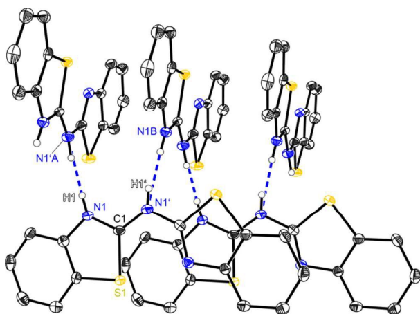
Figure 2. Molecular structure of a hydrogen bridged chain of (NCSC_6H_3)_2NH ( 1 ). Anisotropic displacement parameters are depicted at the 50% probability level. C-H hydrogen atoms are omitted for clarity. Structural data are given in Tables 1–3.
