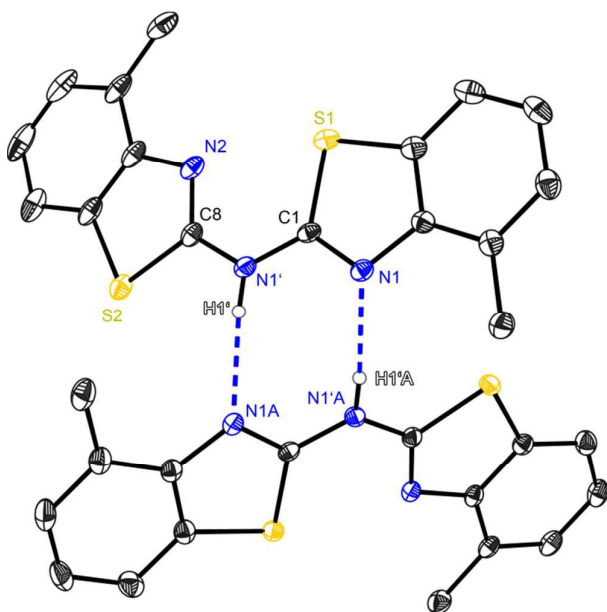
Figure 3. Molecular structure of a hydrogen bridged dimer of (4-Me-NCSC_6H_3)_2NH ( 2 ). Anisotropic displacement parameters are depicted at the 50% probability level. C-H hydrogen atoms are omitted for clarity. Structural data are given in Tables 1–3.
