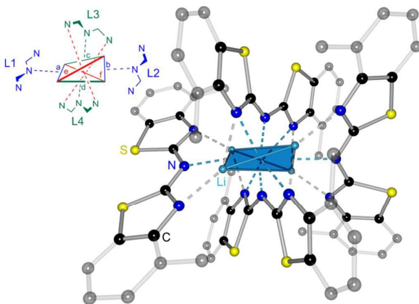
Figure 8. Molecular structure of [\text{Li}((4\text{-Me-NCSC}_6\text{H}_3)_2\text{N})_4] ( 8 ). To clarify the binding motif co-crystallised solvent molecules and hydrogen atoms are omitted as well as the annulated moieties are represented in faded colour. In the upper left corner a simplified model of the coordination environment is depicted.
