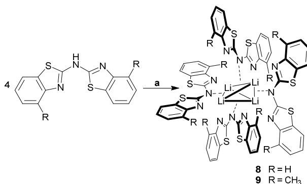
Scheme 7. Synthesis of the lithiated compounds 7–8 (a: 4.4 eq. n BuLi, toluene, 0 °C).
