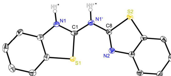
Figure 1. Molecular structure of (NCSCH_4)_2NH ( 1 ). Anisotropic displacement parameters are depicted at the 50% probability level. C–H hydrogen atoms are omitted for clarity. Both hydrogen atoms of the amine moieties highlighted with a star are only partially occupied due to their positional disorder. Structural data are given in Tables 1–3.
