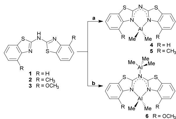
Scheme 5. Synthesis of the dimethyl aluminium containing compounds 4 – 6 (toluene, 0 °C; a: 1.1 eq. \text{AlMe}_3 ; b: exc. \text{AlMe}_3 ).
