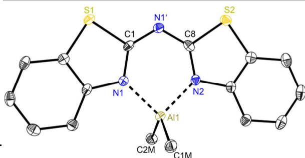
Figure 5. Molecular structure of one molecule of [\text{Me}_2\text{Al}\{(\text{NCSC}_6\text{H}_4)_2\text{N}\}] ( 4 ). Anisotropic displacement parameters are depicted at the 50 % probability level. Hydrogen atoms and positional disorder of the whole molecule are omitted for clarity. Structural data are given in Table 1 and 3.
