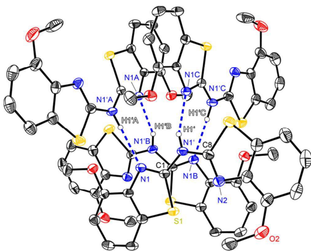
Figure 4. Molecular structure of a hydrogen bridged tetramer of (4-OMe-NCSC_6H_3)_2NH ( 3 ). Anisotropic displacement parameters are depicted at the 50% probability level. C-H hydrogen atoms are omitted for clarity. Structural data are given in Tables 1–3.
