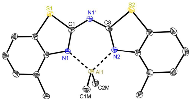
Figure 6. Molecular structure of [Me 2 Al{(4-Me-NCSC 6 H 3 ) 2 N}] ( 5 ). Anisotropic displacement parameters are depicted at the 50 % probability level. Hydrogen atoms are omitted for clarity. Structural data are given in Table 1 and Table 3.
