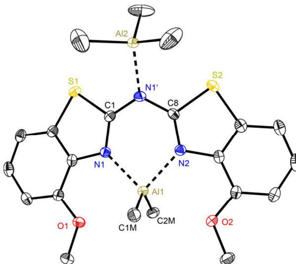
Figure 7. Molecular structure of [Me 2 Al{(4-OMe-NCSC 6 H 3 ) 2 N} · AlMe 3 ] ( 6 ). Anisotropic displacement parameters are depicted at the 50 % probability level. Co-crystallised solvent molecules, hydrogen atoms and positional disorder of the whole molecule are omitted for clarity. Structural data are given in Table 1 and Table 3.
