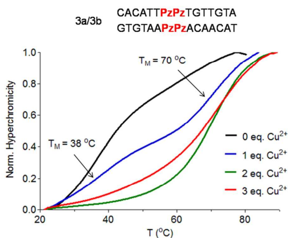
Fig. 4 Schematic depiction of the investigated duplex 3a/3b and \text{Cu}^{2+} titration melting profiles of duplex 3a/3b (Pz = Pyrazole). Conditions: 150 mM NaCl, 10 mM CHES buffer pH 9.0, 1 \mu\text{M} oligonucleotide, final volume of 200 \mu\text{L} .
