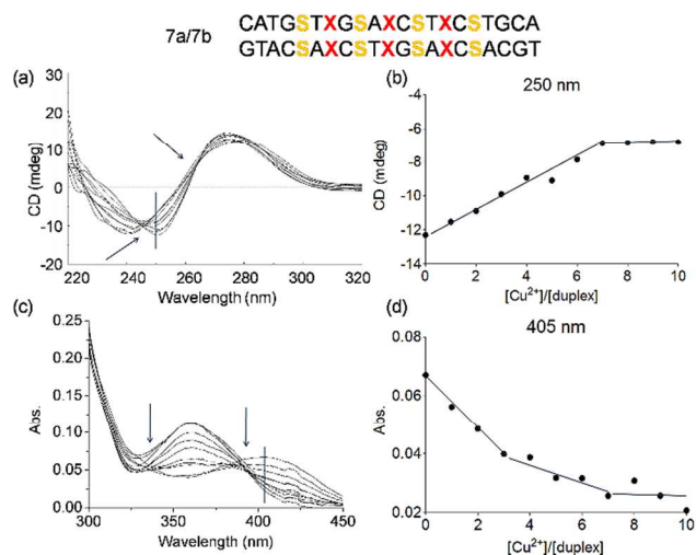
Fig. 8 Schematic depiction of the investigated duplex, S = salen, X = pyrazole. (a) Overlaid CD spectrum at different concentrations of Cu^{2+} (from 0 to 10 eq.) of the duplex 7a/7b ; (b) Plot of circular dichroic changes at 250 nm against the ration of [Cu^{2+}]/[7a/7b] ; (c) Overlaid UV spectrum under the same conditions as in (a); (d) Plot of
