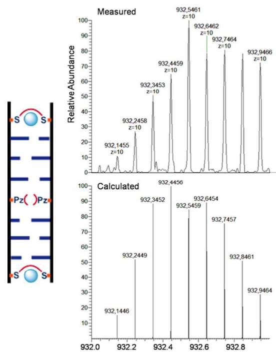
Fig. 7 ESI-Mass spectrum and comparison of experimental data with calculated molecular weights of duplex 6a/6b with 2 eq. \text{Cu}^{2+} , molecular formula
