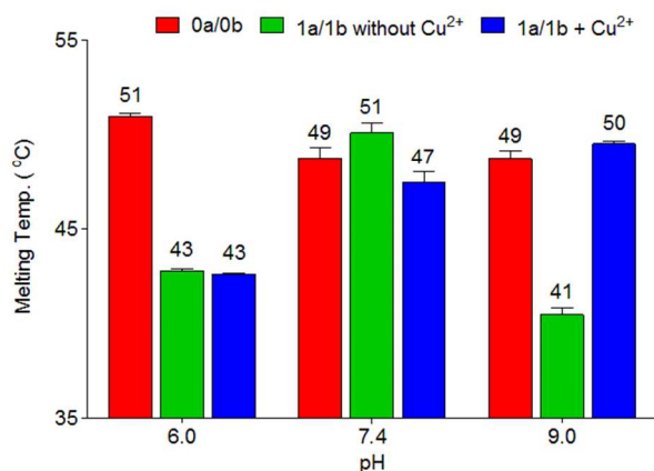
Fig. 2 Melting temperatures of duplexes 0a/0b and 1a/1b at different pH values. Conditions: 150 mM NaCl, 10 mM \text{Na}_2\text{HPO}_4/\text{NaH}_2\text{PO}_4 buffer pH 6.0 / 7.4 or CHES buffer pH 9.0, 1 \mu\text{M} oligonucleotide, with or without 1 \mu\text{M} \text{Cu}^{2+} , final volume of 200 \mu\text{L} .
