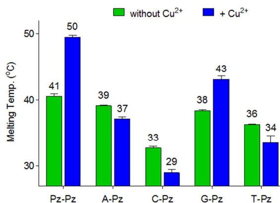
Fig. 3 Melting temperatures of 1a combined with different counter strands having A, G, C, T or Pz as the counter base. Conditions: 150 mM NaCl, 1 mM CHES buffer pH 9.0, 1 \mu\text{M} oligonucleotide, with or without 1 \mu\text{M} \text{Cu}^{2+} , final volume of 200 \mu\text{L} .
