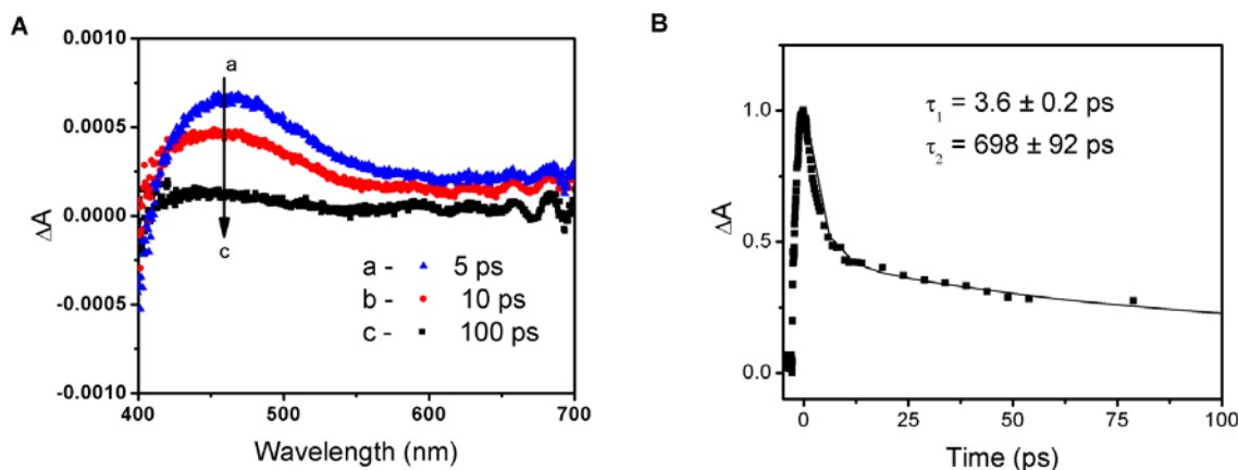
Figure 2. A) Time-resolved transient absorption spectra recorded following 387 nm laser pulse excitation of methylammonium lead iodide precursor solution with 250 \mu\text{M} \text{PbI}_2 and 24 mM MAI in dimethylformamide and B) Absorption–time profile of the induced absorption for the same precursor solution monitored at 500 nm (the difference absorption maximum is normalized to value 1).
