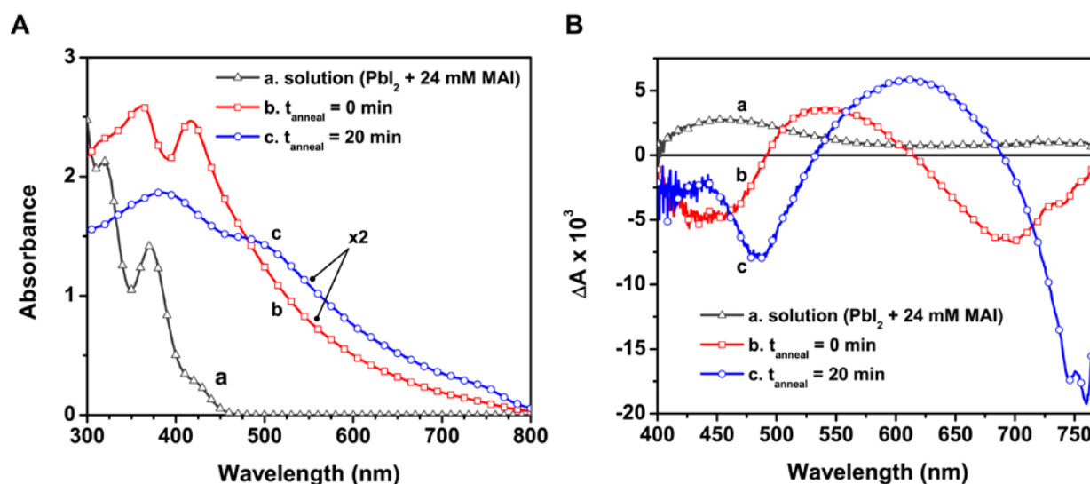
Figure 3. A) Ground state absorption spectra of (a) the perovskite precursor solution in DMF, (b) as-deposited film from a 1:1 \text{CH}_3\text{NH}_3\text{I}:\text{PbI}_2 solution on alumina, and (c) after annealing the deposited film at 100^\circ\text{C} for 20 min. B) Excited state spectra of the same samples recorded 5 ps after 387 nm femtosecond laser pulse excitation in an evacuated cell.
