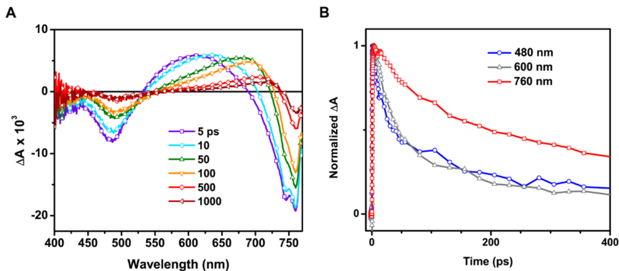
Figure 4. (A) Transient absorption spectra recorded following 387 nm excitation of annealed CH 3 NH 3 PbI 3 on a mesoporous alumina support at various pump-probe delay times. (B) Difference absorption-time profiles recorded at 480 (blue trace), 600 (grey trace), and 760 nm (red trace).
