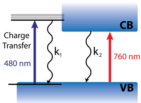
Figure 5. Scheme illustrating the dual nature of the organic-inorganic perovskite excited state.
