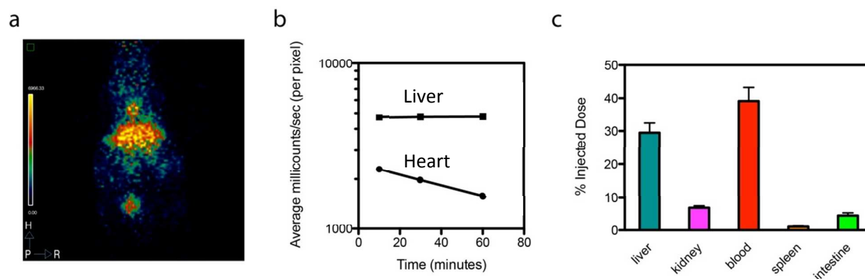
Figure 3 a) PET reconstruction (coronal slice) after injection of 50μCi of 68 Ga dextran tetrazine. b) time-activity curves of liver (squares) and heart (circles). c) Biodistribution of tetrazine dextran after sacrifice.
