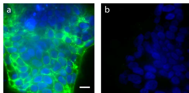
Figure 2. Confocal images of cells treated with fluorescent AlexaFluor 647 (AF647) tetrazine DTPA dextran. A) Cells pretargeted with trans -cyclooctene anti-A33 (sample). Scale bar (lower right) 15 microns. B) Cells lacking A33/TCO (control).
