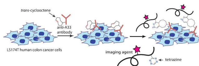
Figure 1: Bioorthogonal inverse Diels-Alder reaction between tetrazine and trans -cyclooctene for multistep labeling of cancer cells with tetrazine DTPA dextran containing an imaging agent.
