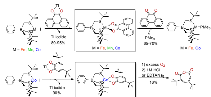
Scheme 1 Synthetic routes to [PhTt tBu ]M(SQ) complexes (M = Fe, Mn, Co) and O 2 reactivity of [PhTt tBu ]Co(3,5-DBSQ).
