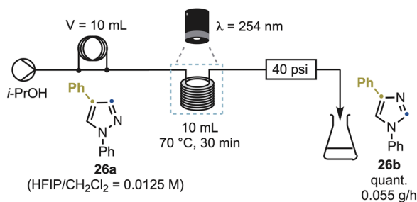
Scheme 7 Reaction scale-up using photo-flow equipment. a Reaction conducted at 0.025 M instead of 0.0125 M. nd: not determined.
