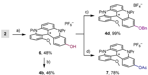
Scheme 4 (a) (i). BBr 3 (5.0 equiv.), CH 2 Cl 2 , 0 to 20 °C, 72 h; (ii) anion metathesis with KPF 6 (aq.). (b) Cs 2 CO 3 (2.5 equiv.), PrI (20 equiv.), DMF, 20 °C, 40 h. (c) (i). Cs 2 CO 3 (2.5 equiv.), BnBr (20 equiv.), DMF, 20 °C, 2.5 h; (ii) anion metathesis with NaBF 4 (aq.). (d) Et 3 N (2.0 equiv.), AcCl (3.0 equiv.), CH 2 Cl 2 , 20 °C, 15 min.
