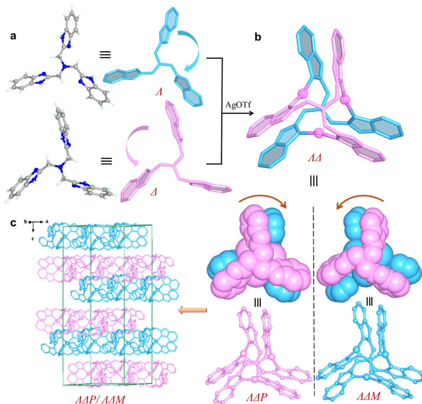
Fig. 1 Racemic crystal structure of 1. (a) \Delta - and \Delta^1 -L 1 . (b) \Delta\Delta P - and \Delta\Delta M -[ \text{Ag}_3\text{L}^2 ] ^{3+} . (c) \Delta\Delta P -[ \text{Ag}_3\text{L}^2 ] ^{3+} and \Delta\Delta M -[ \text{Ag}_3\text{L}^2 ] ^{3+} align alternately along the c axis.
