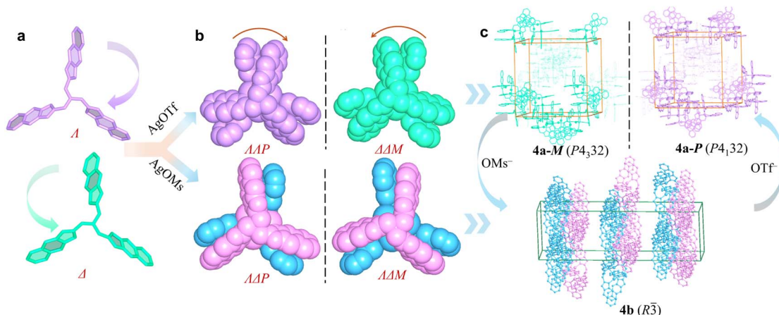
Fig. 4 Anion-induced transition between 4a and 4b. (a) L- and Δ-L 4 . (b) Two pairs of enantiomers of [Ag 3 L 2 ] 3+ (ΔΔP- and ΔΔM-[Ag 3 L 2 ] 3+ , ΔΔP- and ΔΔM-[Ag 3 L 2 ] 3+ ). (c) Anion-induced reversible transition between 4a and 4b.
