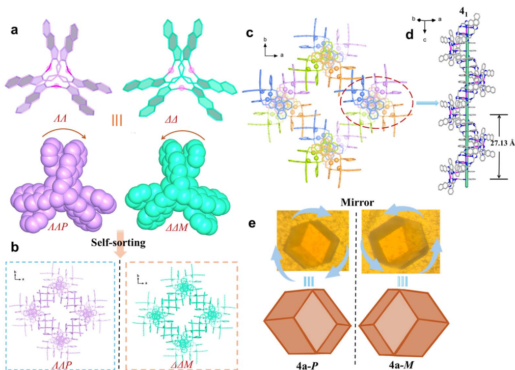
Fig. 3 Crystal structure of 4a . (a) \Delta\Delta - and \Delta\Delta -[Ag 3 L 42 ] 3+ in 4a-P or 4a-M . (b) Narcissistic self-sorting of [Ag 3 L 42 ] 3+ forming chiral structures of 4a-P and 4a-M . (c) Chiral srs network of 4a-P . (d) 4_1 \pi -stacked helical column along the c axis. (e) The photos of 4a-P/4a-M crystals.
