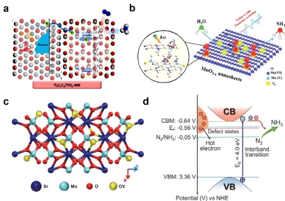
Fig. 8 (a) Schematic illustration of the electronic structures for \text{Ti}_3\text{C}_2\text{T}_x/\text{TiO}_2\text{-400} . Reproduced with permission. 68 Copyright 2020, Elsevier. (b) Schematic illustration of plasmonic photocatalytic \text{N}_2 fixation over \text{MoO}_{3-x} . Reproduced with permission. 69 Copyright 2020, The Royal Society of Chemistry. (c) The structure of \text{SrMoO}_4 with oxygen vacancies. (d) The mechanism for plasmonic photocatalytic nitrogen fixation over \text{SrMoO}_4 with oxygen vacancies. Reproduced with permission. 70 Copyright 2021, Elsevier.
