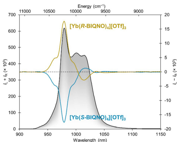
Fig. 4 CPL spectra of [\text{Yb}(\text{S-BIQNO})_4][\text{OTf}]_3 (blue) and [\text{Yb}(\text{R-BIQNO})_4][\text{OTf}]_3 (yellow) in solution in 1,2-difluorobenzene ( 160 \mu\text{M} ). The total luminescence is traced in the background. Excitation: 365 nm, bandpass: 10 nm. B_{\text{CPL}} determined to be 16.1 \text{ M}^{-1} \text{ cm}^{-1} .
