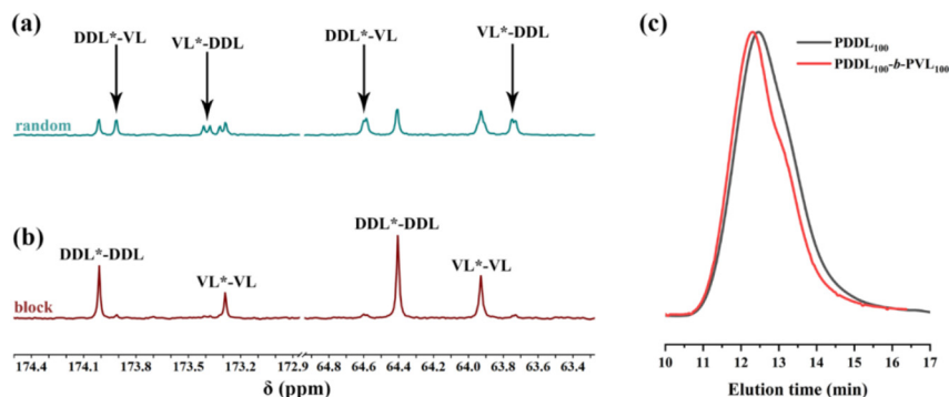
Fig. 7 ^{13}\text{C} NMR spectra of (a) PDDL- ran -PVL (Table S5, run 3) and (b) PDDL- b -PVL (Table 4, run 5), solvent: \text{CDCl}_3 ; (c) GPC curves of the PDDL homopolymer ( T = 130\text{ }^\circ\text{C} , monomer conversion was 80%, M_n = 30.1\text{ kDa} , D = 1.74 ) and copolyesters (Table 4, run 5).
