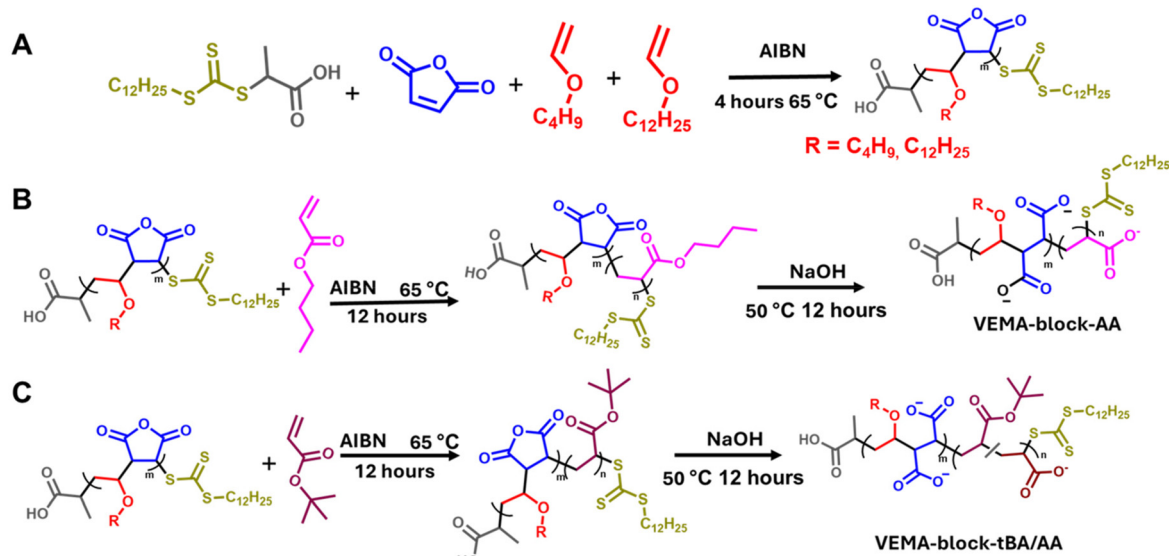
Scheme 1 (A) Synthesis of VEMA copolymers using RAFT copolymerization of vinyl ether and maleic anhydride (B) addition of n -butyl acrylate block in VEMA and hydrolysis to synthesize VEMA- block -AA polymers (C) addition of tert -butyl acrylate block in VEMA and hydrolysis to synthesize the mixture of VEMA- block - t BA and VEMA- block -AA polymers.
