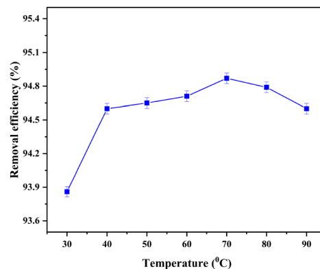
Fig. 11 Effect of temperature on Pb(II) removal by the AOR-C3 film.
