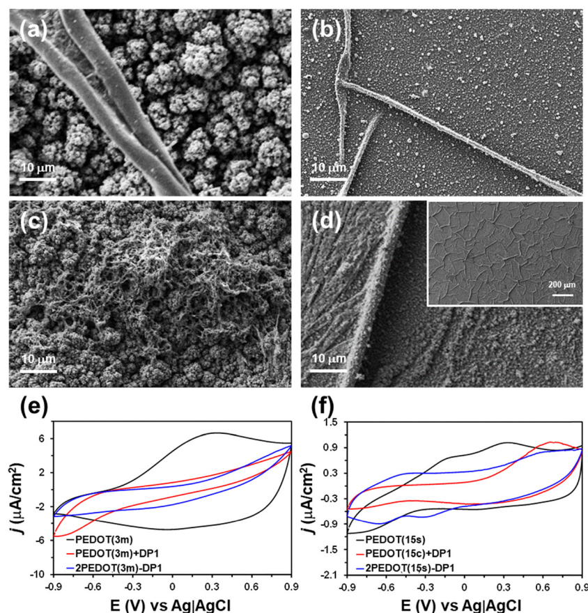
Fig. 2 Representative SEM micrographs of DP1 fibers formed on the surface of (a) PEDOT(3m) and (b) PEDOT(15s) films by dropping 100 \mu L of a 8 mg mL -1 DP1 solution in 40 : 60 HFIP : H 2 O. (c and d) Representative SEM micrographs of (c) 2PEDOT(3m)- DP1 and (d) 2PEDOT(15s)- DP1 three-layered electrodes. Cyclic voltammograms recorded for pristine PEDOT films, PEDOT films with DP1 fibers on the surface (PEDOT + DP1 ) and 2PEDOT- DP1 electrodes, where PEDOT films were prepared using a t_p of (e) 3 min and (f) 15 s.
