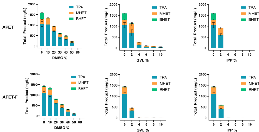
Fig. 4 LCC IGG tolerance to organic solvents dimethyl sulfoxide (DMSO), gamma-valerolactone (GVL), and 2-isopropylphenol (IPP) at varying concentrations on an amorphous PET film (APET-F) and powder (APET). Enzyme activity was assessed using two known enzymatic hydrolysable substrates, APET and APET-F. Solvent concentrations ranged from 0% to 100% in 10% increments; however, due to a marked reduction in activity at higher concentrations of GVL and IPP, detailed analysis was focused on the 0% to 10% range in 2% increments for these solvents. Total degradation products released from PET hydrolysis were quantified by high-performance liquid chromatography (HPLC). Monomers TPA, MHET, and BHET released are shown as mean values with standard deviation (SD) from replicate experiments, with TPA in blue, MHET in orange, and BHET in green.
