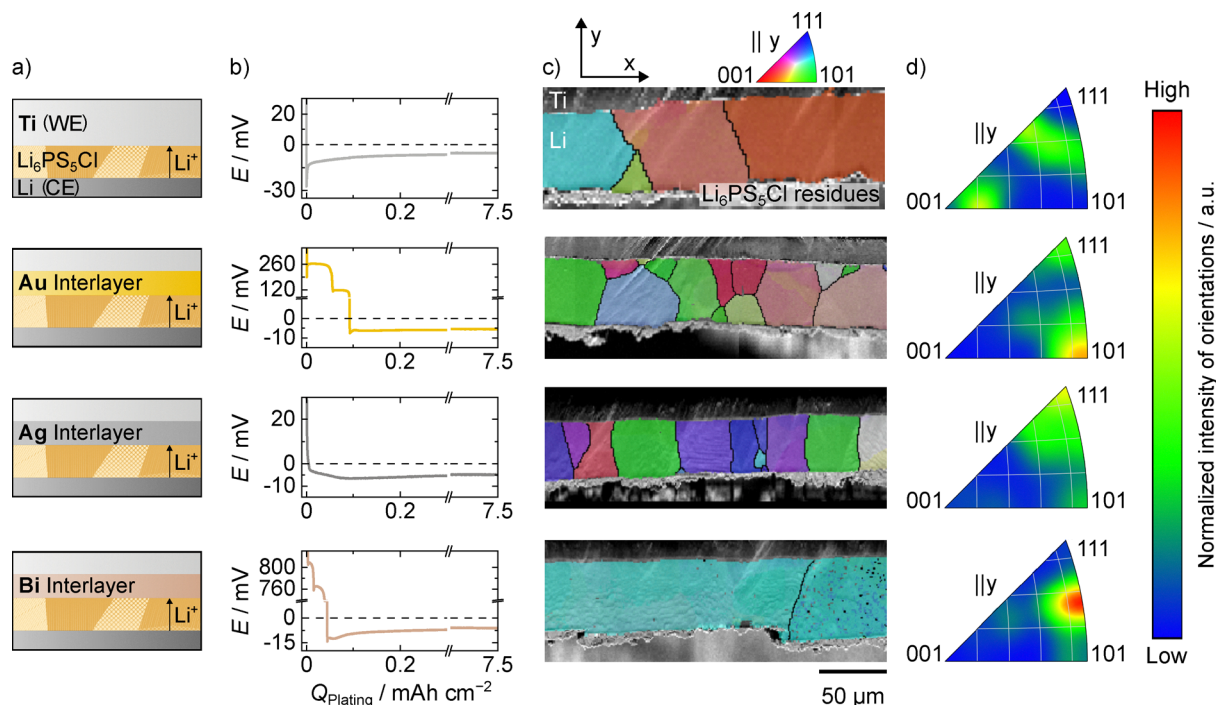
Fig. 1 Electrodeposition of lithium using (a) different interlayer materials. (b) Voltage profiles of the respective cell systems ( T = 25^\circ\text{C} , j = 150 \mu\text{A cm}^{-2} ). As schematically depicted, titanium was used as reference (top row) and gold (2nd row), silver (3rd row) and bismuth (4th row) were used as interlayer materials. (c) Microstructure of the electrodeposited lithium layers using the different interlayer materials. The IPF maps are given parallel to the y -direction as indicated above. The shown scalebar represents 50 \mu\text{m} in all cases. (d) IPFs of the analyzed cross-sections showing the distribution of the orientation of all analyzed grains. The IPFs are given parallel to the y -direction. Please note that the IPFs were created based on the entire analyzed cross-section, which is shown in the SI.
