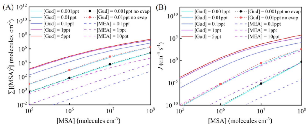
Fig. 7 Variation of simulated steady-state MSA dimer concentration \Sigma[(\text{MSA})_2] (molecules per \text{cm}^3 ) (A) and cluster formation rate J ( \text{cm}^3 \text{s}^{-1} ) (B) with monomer concentration at 278.15 K and \text{CoagS} = 2.6 \times 10^{-3} \text{s}^{-1} . Adapted from Liu et al. , 2022. 62 Reproduced from ref. 62 with permission from the American Chemical Society, copyright 2022.
