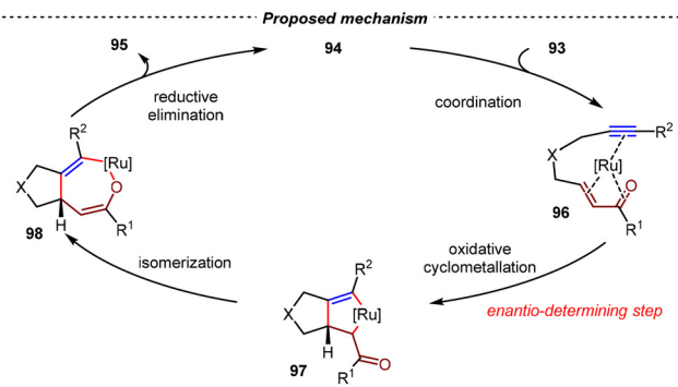
Scheme 24 Ruthenium (II)-catalyzed asymmetric intramolecular [4+2] cycloadditions of yne-enones.
