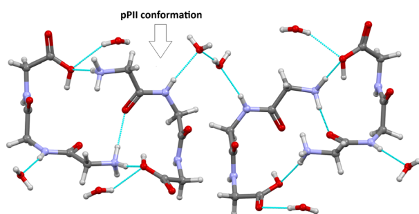
Fig. 1 Hydration-stabilised extended pPII conformation in triglycine ( \text{GGG}\cdot 2\text{H}_2\text{O} ). The structure highlights the water-mediated hydrogen-bond network stabilising the extended peptide backbone. Crystal structure data were obtained from the Cambridge Structural Database (CSD, refcode ZZZPTQ01).
