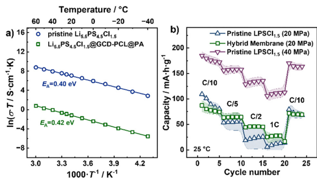
Fig. 4 (a) Arrhenius plot of the infiltrated membrane \text{LPSCl}_{1.5}@\text{GCD-PCL}@\text{PA} with activation energy E_A = 0.42 eV and pristine \text{LPSCl}_{1.5} with activation energy E_A = 0.40 eV. (b) Discharge capacities of the rate-performance test in a Li/In half-cell setup at 20 MPa and 40 MPa, where 1\text{C} = 180 \text{ mAh g}^{-1} .
