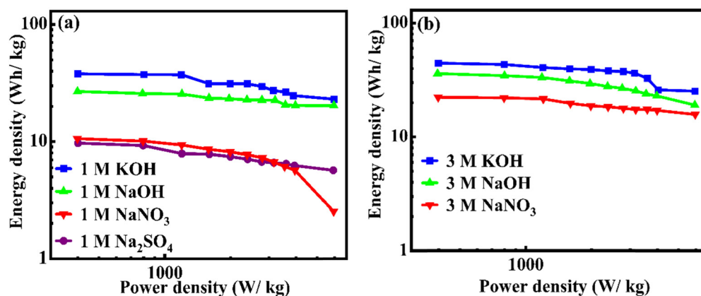
Fig. 17 Ragone plot of Mn_2O_3 -9 in (a) 1 M and (b) 3 M concentrations of electrolytes measured at a current density range from 1 to 15\text{ A g}^{-1} .
