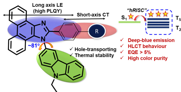
Fig. 1 Molecular design of the PICz-based deep-blue HLCT emitters.
