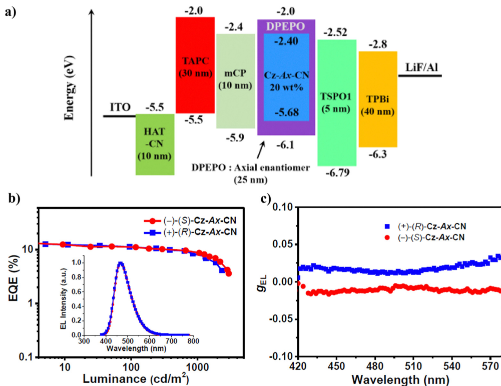
Fig. 17 (a) The energy diagram of CP-OLEDs based on (–)-( S )- 5 and (+)-( R )- 5 . (b) EQE–luminance characteristics. Inset: EL spectra of the devices at 6 V. (c) The g_{\text{EL}} values of the devices as a function of emission wavelength. Reproduced with permission from ref. 32. Copyright 2020, Wiley-VCH.
