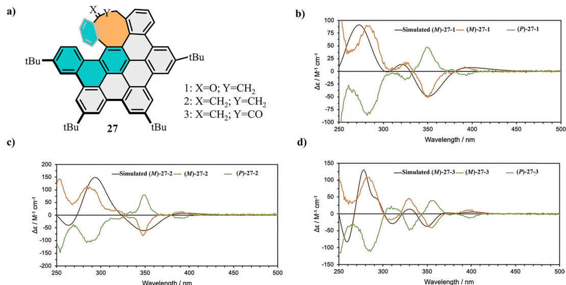
Fig. 12 (a) Schematic diagram of 27 . (b)–(d) Experimental ECD spectra of (M/P)-27-1 to (M/P)-27-3 in DCM, and simulated (CAM-B3LYP/6-311++G(d,p), IEFPCM DCM) ECD spectra of (M)-isomers: (b) (M)-27-1 and (P)-27-1 (orange and green, both 1.2 \times 10^{-5} M), (c) (M)-27-2 (orange, 1.0 \times 10^{-5} M) and (P)-27-2 (green, 1.1 \times 10^{-5} M) and (d) (M)-27-3 (orange, 1.3 \times 10^{-5} M) and (P)-27-3 (green, 1.4 \times 10^{-5} M). Reproduced with permission from ref. 56. Copyright 2021, Wiley-VCH.
