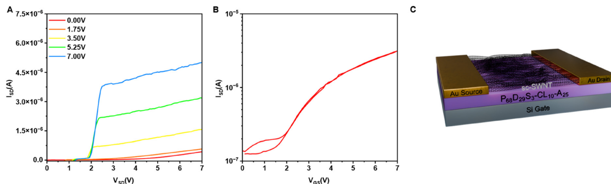
Fig. 4 Characteristic (a) output, (b) transfer curves for BGTC OTFTs prepared using P_{68}D_{29}S_3\text{-CL}_{10}\text{-A}_{25} with sc-SWCNTs. The transfer curve was operated at a V_{SD} of 3V, and the average of the last measurement of five transfer curves is presented to ensure the film is appropriately charged (c) BGTC device architecture.
