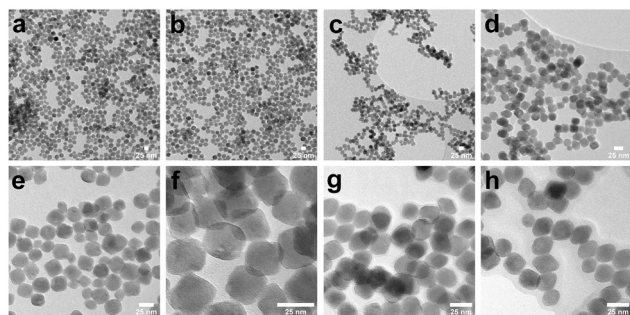
Fig. 2 TEM images of LiLuF_4:Tm^{3+}, Yb^{3+} core nanocrystals with the following lanthanide ratios: (a and e) 1\%Tm^{3+}, 30\%Yb^{3+} ; (b and f) 1\%Tm^{3+}, 35\%Yb^{3+} ; (c and g) 1.5\%Tm^{3+}, 30\%Yb^{3+} ; and (d and h) 1.5\%Tm^{3+}, 35\%Yb^{3+} . The top images show a general overview of the nanocrystals, while the bottom images were obtained at higher magnification. The scale bar is 25 nm for all images.
