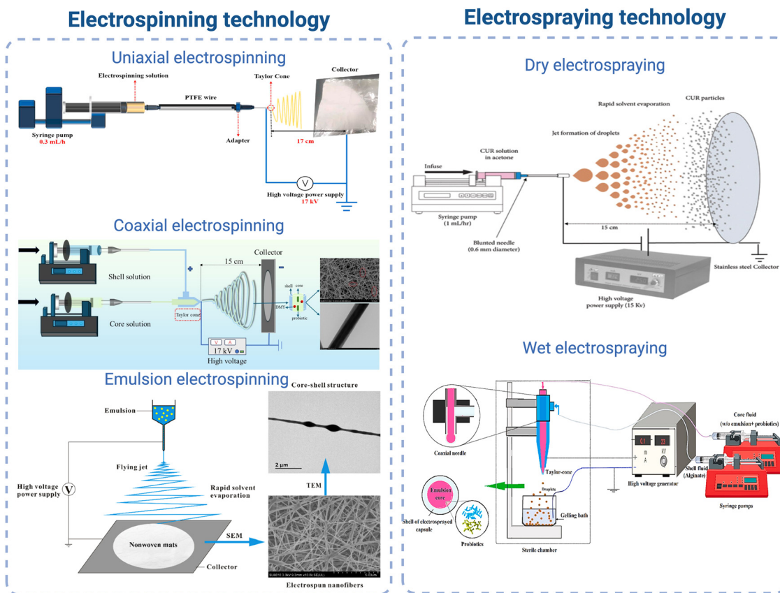
Fig. 8 Overview of electrohydrodynamic techniques, including electrospinning (uniaxial, reproduced from ref. 97 with permission from Elsevier, copyright 2022; coaxial, reproduced from ref. 99 with permission from Elsevier, copyright 2025; and emulsion, reproduced from ref. 154 with permission from Elsevier, copyright 2018) and electrospaying (dry, reproduced from ref. 155 with permission from Wiley, copyright 2024, CC BY 4.0 license; and wet, reproduced from ref. 107 with permission from Elsevier, copyright 2024).
