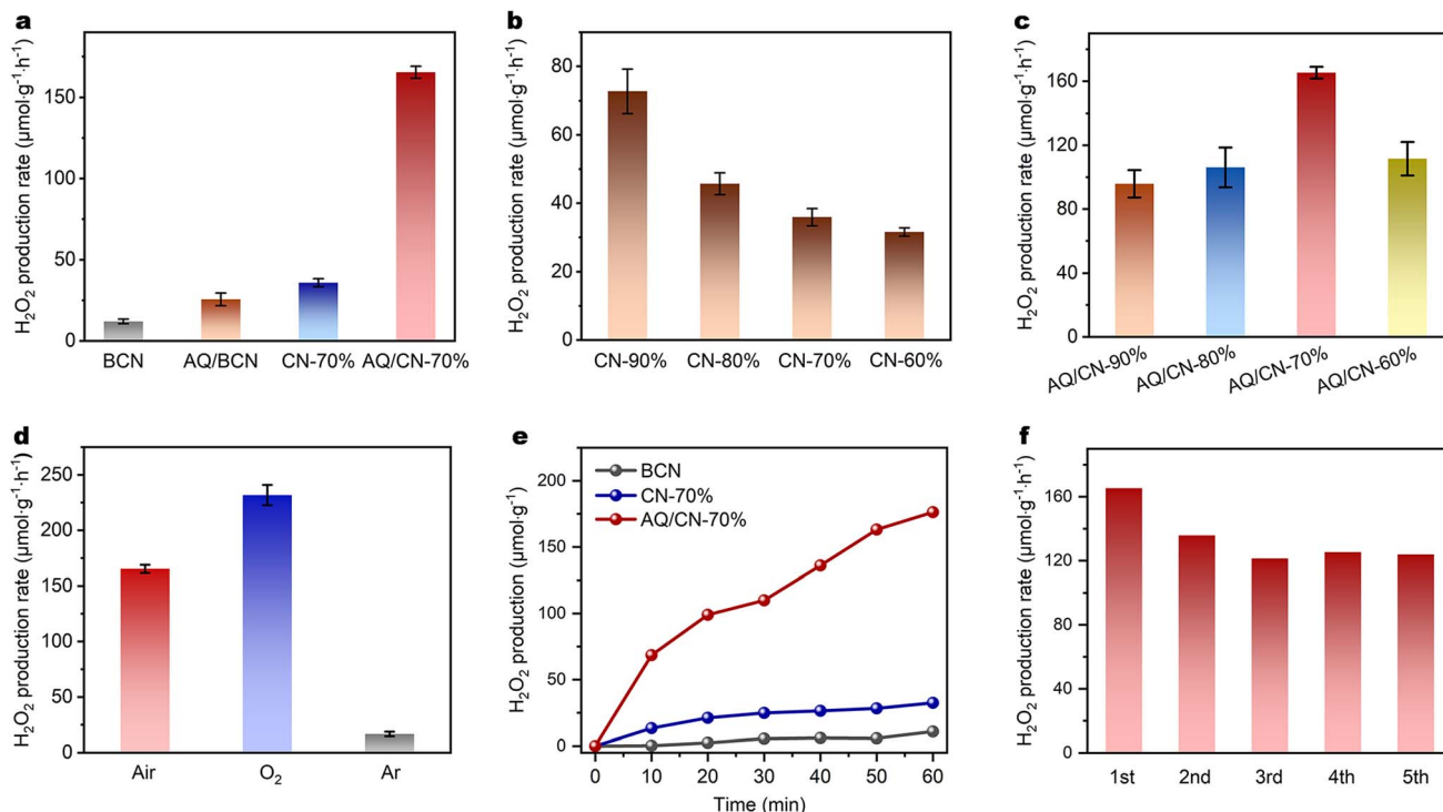
Fig. 2 (a) Photocatalytic H 2 O 2 production rates of BCN, AQ/BCN, CN-70% and AQ/CN-70%, (b and c) H 2 O 2 production rates of CN- x % and AQ/CN- x %, (d) photocatalytic H 2 O 2 production rate of AQ/CN-70% under varying atmospheres, (e) time-dependent H 2 O 2 production kinetics of BCN, CN-70% and AQ/CN-70%, and (f) photocatalytic cycling stability of AQ/CN-70% for H 2 O 2 production. Reaction conditions: 300 W Xenon light source equipped with a cut-off filter ( \lambda \geq 420 nm); irradiation intensity: 300 mW cm -2 ; reaction temperature: 25 °C.
