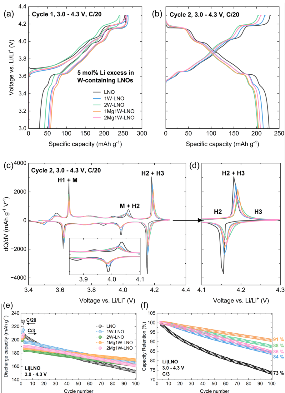
Fig. 7 (a) First and (b) second cycle charge–discharge profiles, (c) second cycle differential capacity (dQ/dV) plots, (d) expanded view of the 4.1 to 4.3 V vs. Li/Li + dQ/dV region encompassing the H2 to H3 transition and comparison of (e) specific discharge capacity stability and (f) normalised discharge capacity retention for LNO, 1W-LNO, 2W-LNO, 1Mg1W-LNO and 2Mg1W-LNO from galvanostatic cycling of half-coin cells between 3.0 and 4.3 V vs. Li/Li + at 25 °C.
