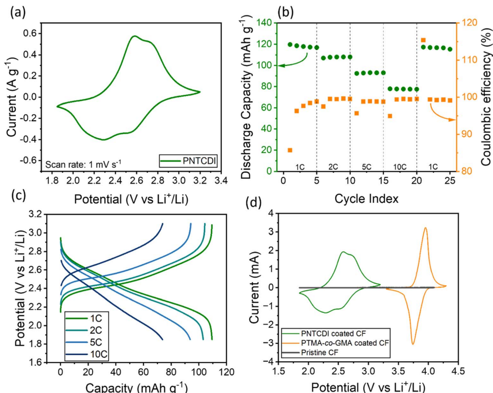
Fig. 2 Electrochemical characteristics of PNTCDI-coated CF in a half cell (vs. lithium foil) at room temperature (24 °C). (a) CV at 1 mV s -1 . (b) Discharge capacity at varying C-rates. (c) GCD curves at different C-rates. (d) CV curves of PNTCDI, PTMA-co-GMA, and neat CF shown together. The electrolyte was 1 M LiTFSI in diglyme/FEC (9 : 1, w : w). All cells had an active material loading of >1 mg cm -2 .
