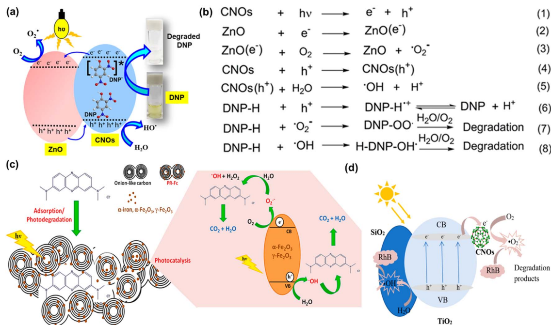
Fig. 11 (a) An illustration of the photodegradation of DNP by the T-ZnO-CNO hybrid composite, (b) a plausible mechanism of the photodegradation of DNP by the T-ZnO-CNO hybrid composite under visible-light irradiation, 85 (c) visual depiction of the synergistic adsorption-photocatalytic processes driving methylene blue degradation by the engineered PR-Fc catalyst, 107 (d) the mechanism diagram of \text{SiO}_2/\text{CNOs}/\text{TiO}_2 in the degradation of dyes in visible light. 81
