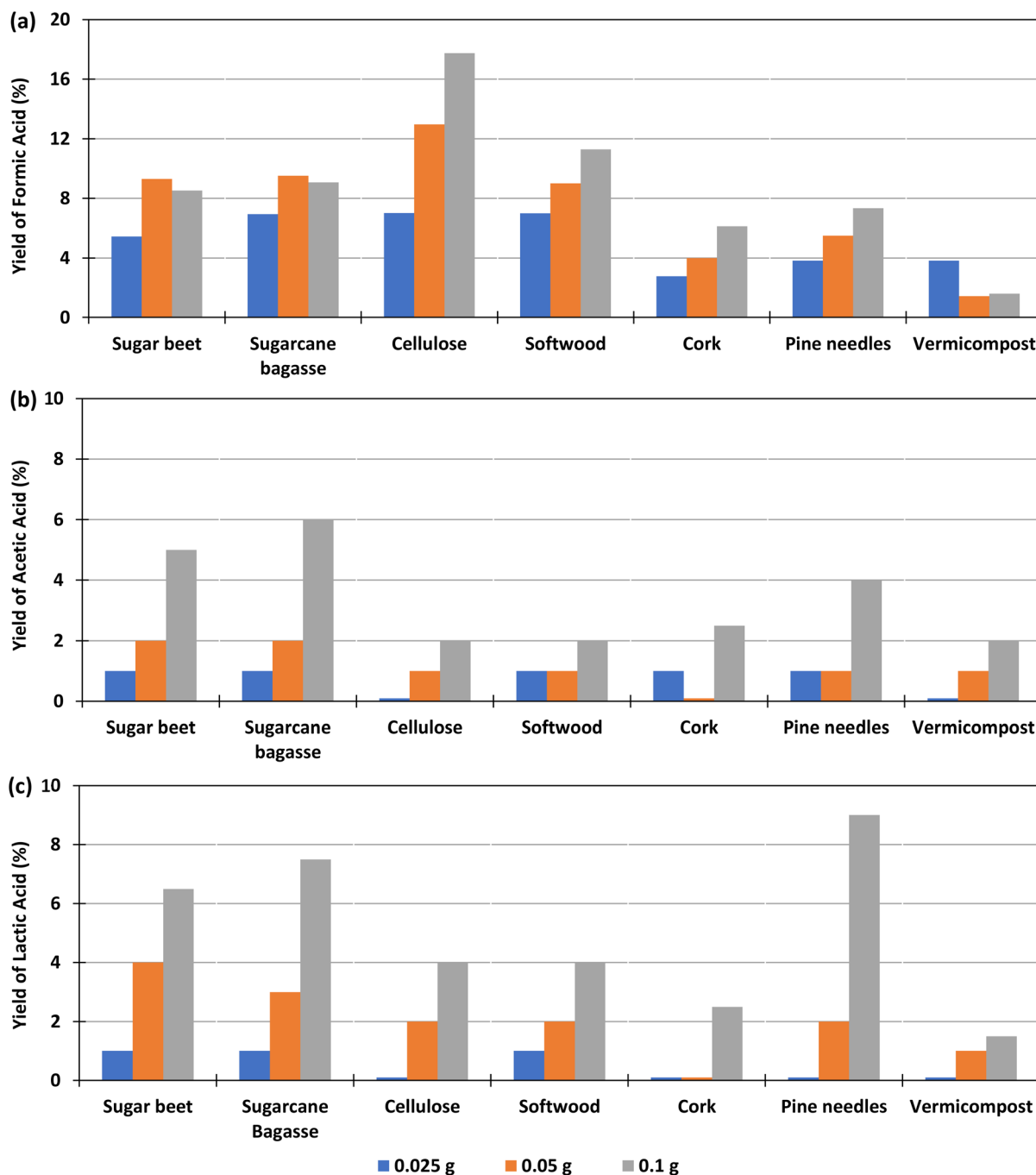
Fig. 5 Effect of different amount of biomass in the yields of formic acid (a); acetic acid (b) and lactic acid (c) in the reaction of \text{HCO}_3^- with biomass. Conditions of reaction: mass ratio Pd(5%)/C : biomass 1 : 1, 2 : 1, and 4 : 1, 0.1 g of catalyst, 0.5 M \text{NaHCO}_3 , 45% filling volume of reactor, 300 °C, 2 h.
