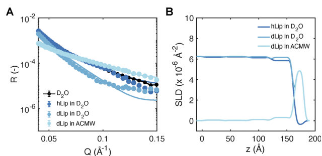
Fig. 3 Structure of a lipid mixture: (A) specular neutron reflectivity ( R ) as a function of momentum transfer vector ( Q ) for hLip in D 2 O, dLip in D 2 O, and dLip in ACMW at 36.5 ^{\circ}\text{C} . The reflectivity curve for pure D 2 O is shown in black. Solid lines represent the multilayer slab model fit. (B) Scattering length density (SLD) profile obtained by the model fit, where the layer thickness ( z ) extends from the buffer–air interface (at z_{\text{max}} ) to the bulk (at z = 0 ).
