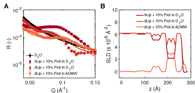
Fig. 5 Increasing protein concentration leads to multilayer formation: (A) specular neutron reflectivity ( R ) as a function of momentum transfer vector ( Q ) for hLip + 10% SP-B + 10% SP-C in \text{D}_2\text{O} , dLip + 10% SP-B + 10% SP-C in \text{D}_2\text{O} , and dLip + 10% SP-B + 10% SP-C in ACMW at 36.5^\circ\text{C} . The pure \text{D}_2\text{O} reflectivity curve is shown in black. Solid lines represent the multilayer slab model fit. (B) Scattering length density (SLD) profile obtained from the model fit, where the layer thickness ( z ) extends from the buffer–air interface ( z_{\text{max}} ) to the bulk ( z = 0 ).
