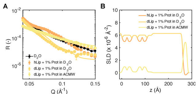
Fig. 4 The effect of physiological amounts of SPs: (A) specular neutron reflectivity ( R ) as a function of momentum transfer vector ( Q ) for hLip + 1% SP-B + 1% SP-C in \text{D}_2\text{O} , dLip + 1% SP-B + 1% SP-C in \text{D}_2\text{O} , and dLip + 1% SP-B + 1% SP-C in ACMW at 36.5^\circ\text{C} . The pure \text{D}_2\text{O} reflectivity curve is shown in black. Solid lines correspond to the multilayer slab model fit. (B) Scattering length density (SLD) profile obtained by the model fit, where the layer thickness ( z ) extends from the buffer–air interface ( z_{\text{max}} ) to the bulk ( z = 0 ).
