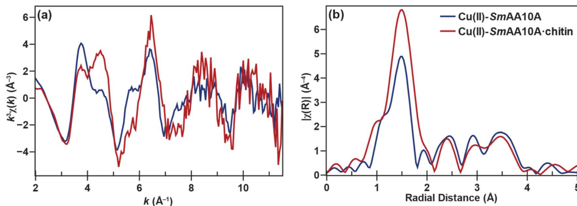
Fig. 4 (a) k^3 -weighted EXAFS and (b) FT-EXAFS of \text{SmAA10A-Cu(II)} (blue) and \text{SmAA10A}\cdot\text{Cu(II)-chitin} (red). Data for the chitin-bound spectrum is derived from the 75% chitin-bound sample following subtraction.
