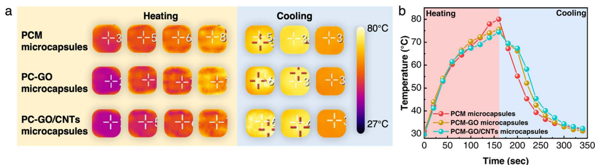
Fig. 5 (a) Infrared thermographic images and (b) plots of temperature evolution as a function of time for PCM microcapsule, PCM-GO microcapsules and PCM-GO/CNTs microcapsules.
