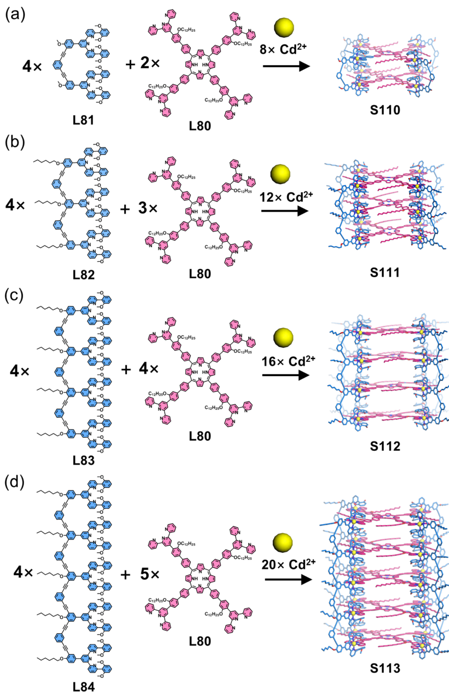
Fig. 43 (a) Simulated structure of cage S110 assembled from ligands L80 and L81 . (b) Simulated structure of cage S111 assembled from ligands L80 and L82 . (c) Simulated structure of cage S112 assembled from ligands L80 and L83 . (d) Simulated structures of cage S113 assembled from ligands L80 and L84 .
