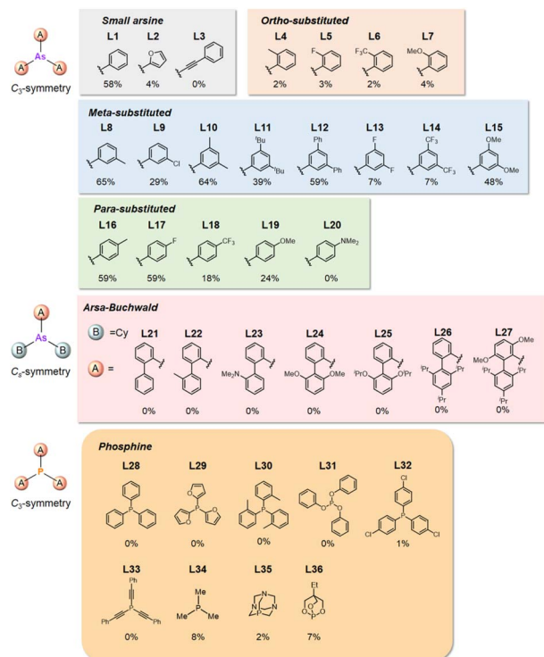
Fig. 2 o -, m -, and p -substituted C_3 - and C_s -type arsine and phosphine ligands. The NMR yield of the difunctionalized product 1 (Scheme 1) is shown below each structure.
