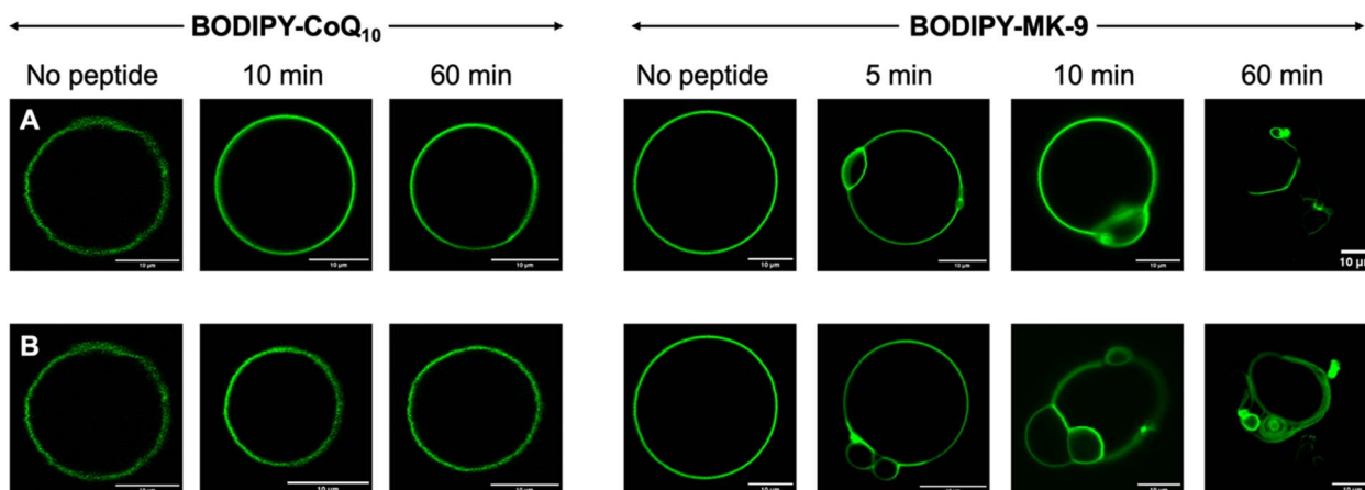
Fig. 3 Fluorescence microscopy of GUVs containing BODIPY-PPQs. Row (A) shows effects of Hex-MBA2 addition and row (B) shows effects of Hex-LysE addition. Laser excitation wavelength = 488 nm, emission detection wavelength = 496–669 nm. Scale bar 10 μm in all panels.
