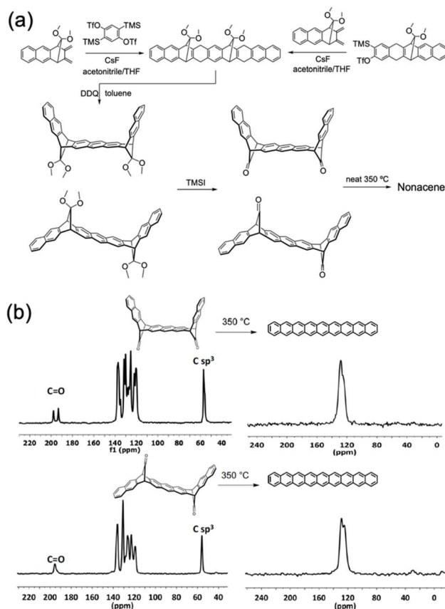
Fig. 26 (a) Synthetic route for nonacene precursors. (b) Thermal decarbonylation of precursors at 350 °C for 20 min and ^{13}\text{C} CP-MAS NMR spectra. Adapted with permission from ref. 99. Copyright 2022 Springer Nature.
