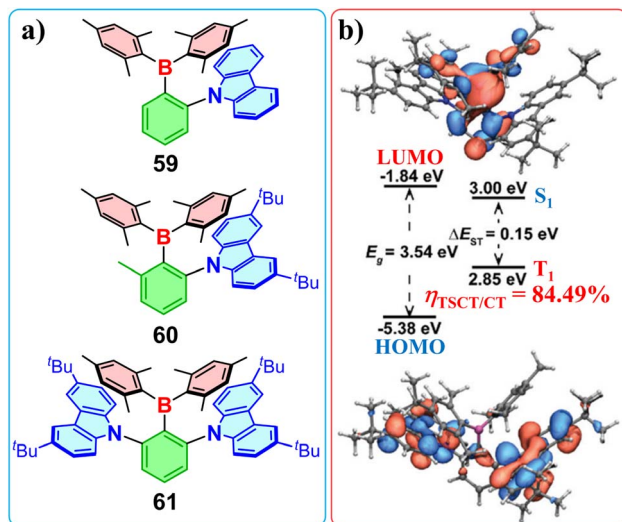
Fig. 18 (a) TADF-emissive TSCT molecules with triarylboron acceptors. (b) The calculated HOMO/LUMO distributions, \Delta E_{\text{ST}} and the TSCT/CT ratio ( \eta_{\text{TSC/CT}} ) for 61. Copyright 2021, The Royal Society of Chemistry.
