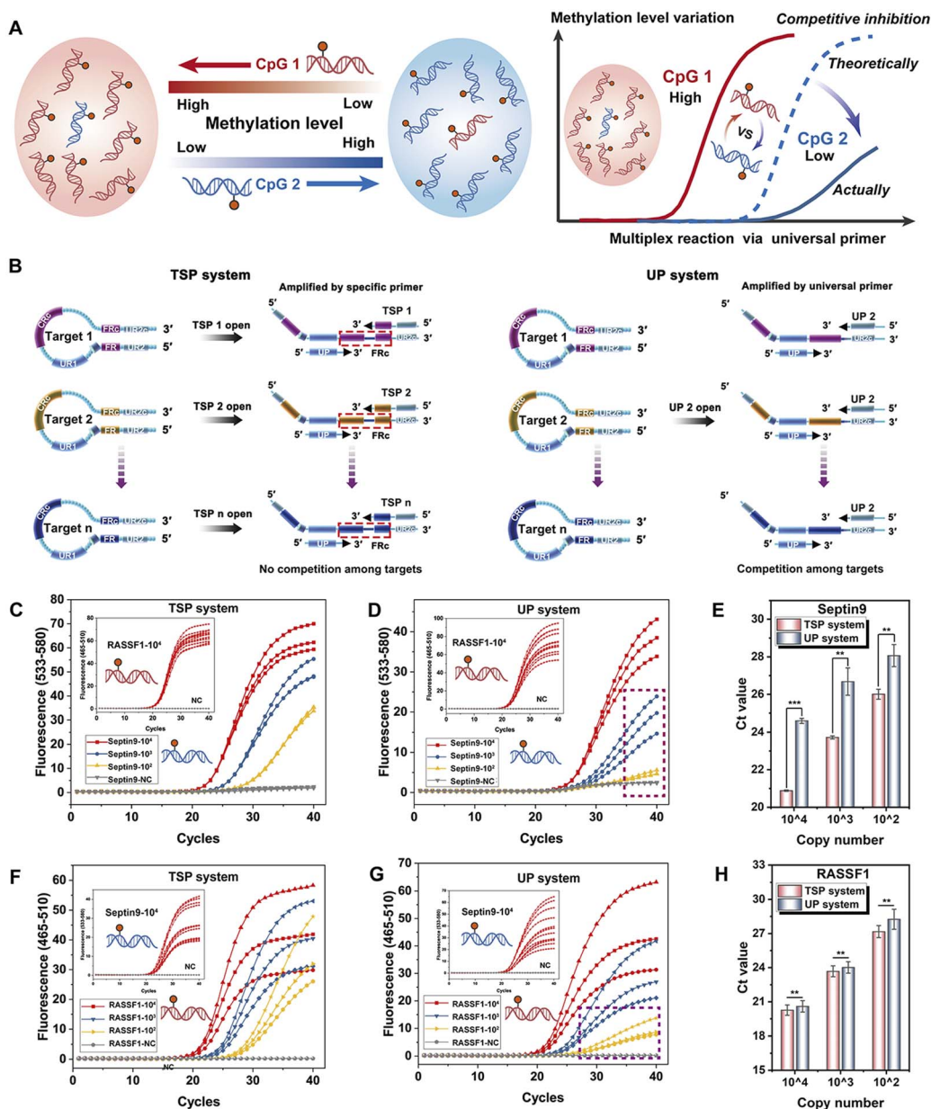
Fig. 5 (A) Diagram illustrating the competitive reactions arising from differential methylation at various sites within a multiplex system. (B) The schema of the TSP system: the different HPs were opened by specific TSPs, and further amplified by TSPs and the UP. The UP system: the different HPs were all opened by UP1, and further amplified by UP1 and UP2. The amplification curves of serially diluted Septin9 methylated plasmid at 10^4 , 10^3 , and 10^2 copies per reaction with a background of 10^4 copies of RASSF1 methylated plasmid in the (C) TSP system and the (D) UP system. (E) Comparison of C_t values from Septin9 at 10^4 , 10^3 , and 10^2 (copies per reaction) within 10^4 of RASSF1 between the TSP and UP systems. The amplification curves of serially diluted RASSF1 methylated plasmid at 10^4 , 10^3 , and 10^2 (copies per reaction) with a background of 10^4 copies of the Septin9 methylated plasmid in the (F) TSP system and the (G) UP system. (H) Comparison of C_t values from RASSF1 at 10^4 , 10^3 , and 10^2 (copies per reaction) within 10^4 of Septin9 between the TSP and UP systems. The data are expressed as the mean \pm SD ( n = 3 ), p -values: ** p < 0.01 , *** p < 0.001 .
