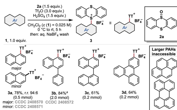
Fig. 1 Current strategies for PAH solubilization and regioselective arene functionalization. (A) Dissolution of PAHs. (B) Regioselective sulfoniumization of small arenes via thianthreneation. (C) This work.
