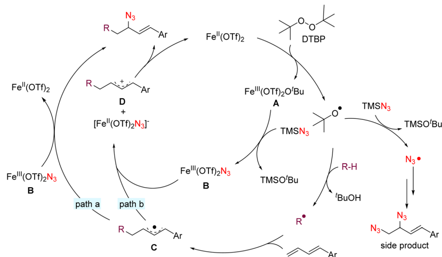
Scheme 4 Proposed catalytic cycle.
