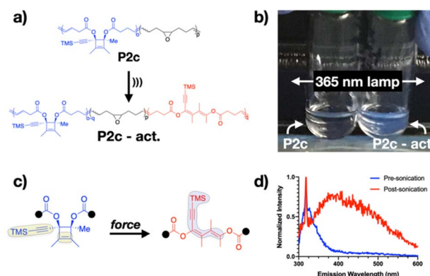
Fig. 5 (a) Sonication of P2c opens the cyclobutene ring, leading to observed fluorescence in the post-sonicated solution (b). The fluorescence is attributed to increased conjugation, including that to the alkyne substituent (c). (d) Emission spectrum of pre- and post-sonication solutions of P2c .
