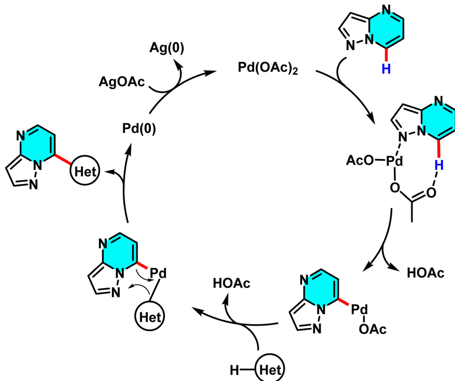
Scheme 24 Proposed pathway for \text{Pd}(\text{OAc})_2 -catalyzed reaction between pyrazolo[5,4- b ]pyridines and five-membered heterocyclic.
