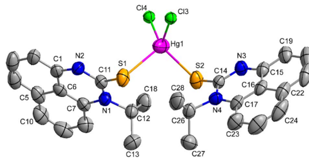
Fig. 1 Molecular structure of mercury(II) complex ( 1 ). Thermal ellipsoids are at a 50% probability level. Hydrogen atoms and solvent molecules are omitted for clarity. Selected bond distances (Å): Hg1–Cl4 2.443(3); Hg1–Cl3 2.448(3); Hg1–S2 2.540(2); Hg1–S1 2.596(2). Bond angles ( ^\circ ): Cl4–Hg1–Cl3 112.76(10); Cl3–Hg1–S2 117.10(9); Cl4–Hg1–S1 113.61(9); S2–Hg1–S1 104.16(7).
