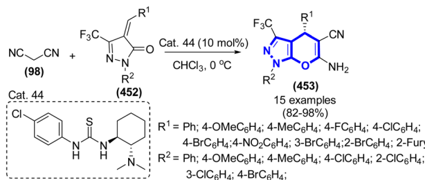
Scheme 121 Synthesis of functionalized dihydropyrano[2,3- c ]pyrazoles catalyzed by Cat. 44.
