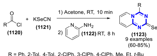
Scheme 309 Synthesis of 2H-pyrido[1,2-a][1,3,5]triazine-2-selenones.
