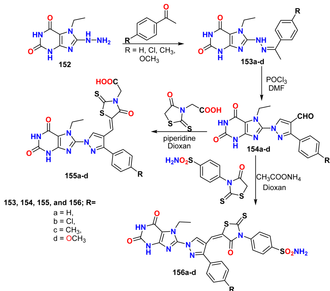
Scheme 41 Synthesis of new Schiff bases based on purine derivatives.
