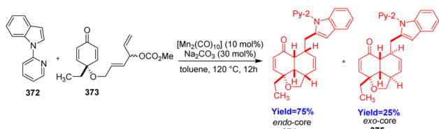
Scheme 47 Synthesis of 6/6/5-fused tricyclic terpenoid scaffold. 101
