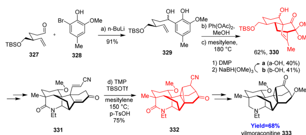
Scheme 42 Total synthesis of vilmoreaconitine (333). 94
