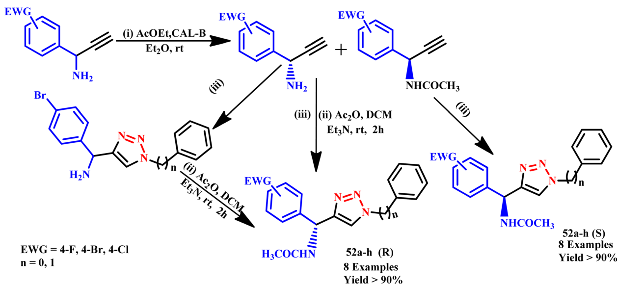
Scheme 41 Microwave-assisted synthesis of a-[4-(1-substituted)-1,2,3-triazol-4-yl]benzylacetamides. Conditions: (iii) (for n = 1 ) \text{NaN}_3 , benzyl chloride, sodium ascorbate/ \text{Cu}(\text{SO}_4) \cdot \text{H}_2\text{O}/\text{BuOH} , MW, 125 °C, 10 min; (for n = 0 ) \text{pHn}_3 , sodium ascorbate/ \text{CuSO}_4 \cdot \text{H}_2\text{O}/\text{BuOH} , MW, 120 °C, 10 min. 82
