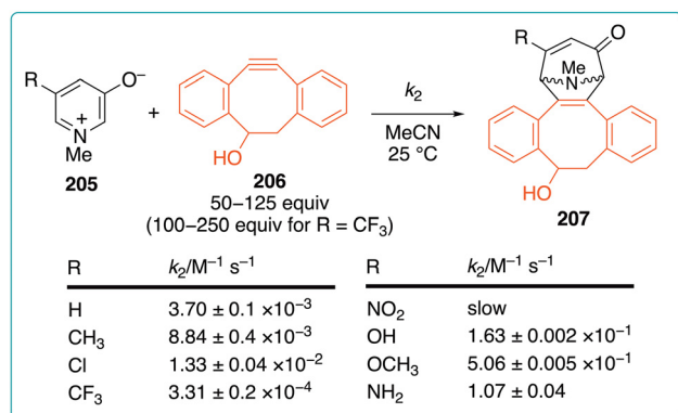
Fig. 30 Kinetic study of the (5 + 2) cycloaddition of oxido-1-methylpyridinium betaines with 4-dibenzocyclooctynol.
